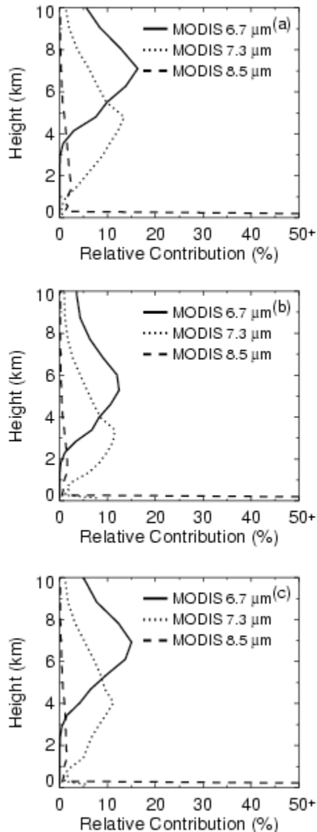
Figure 4. MODIS water-vapor channel contribution functions for mean sounding conditions associated with the main cloud types. (a) Liquid, (b) mixed, Z_{top} < 3 km, and (c) ice, Z_{top} > 3 km.
