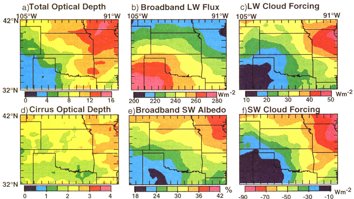
Figure 4. Mean daytime radiative properties derived from GOES-8 during SUCCESS. Cloud forcing and LW flux for 24 hours.
