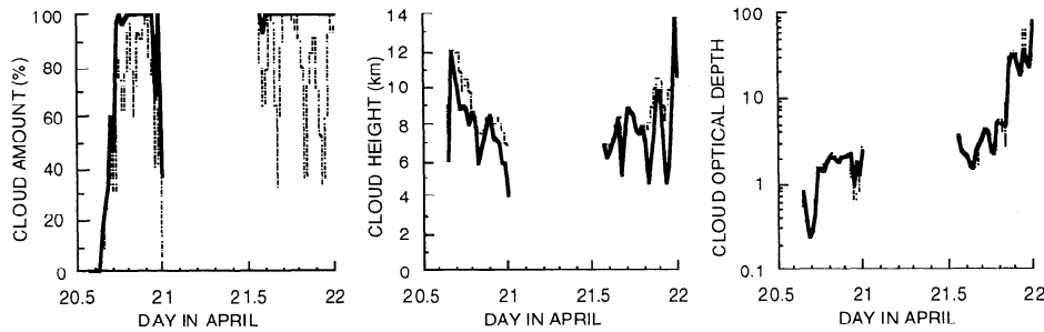
Figure 1. Daytime total (solid) and high (dotted) cloud properties for April 20-21, 1996 over the ARM SCF.
