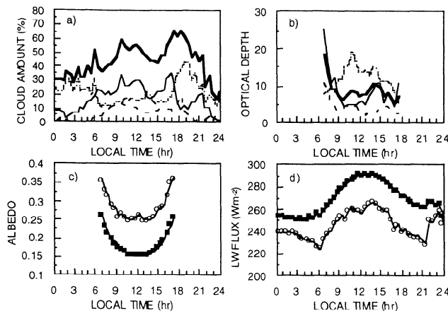
Figure 2. Mean diurnal variation of cloud and radiative parameters over SCF 0.3^\circ box during SUCCESS (April 9 - May 9, 1996) for low (dotted), midlevel (long dash), high (thin solid), and total (heavy solid) clouds and clear (solid symbols) and total (open symbols) albedo and LW flux.
